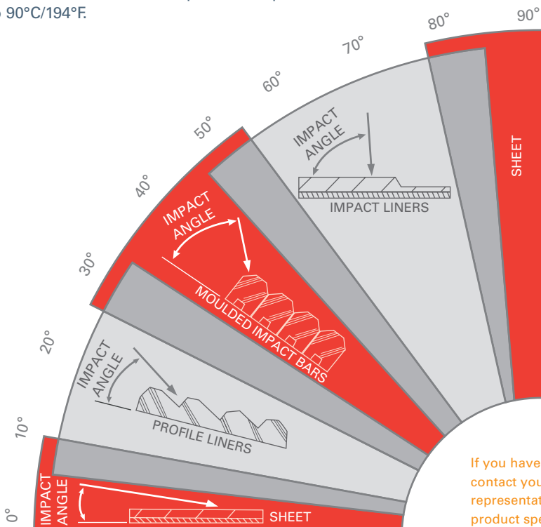
Selection Criteria for Impact Angle and Sliding Wear
